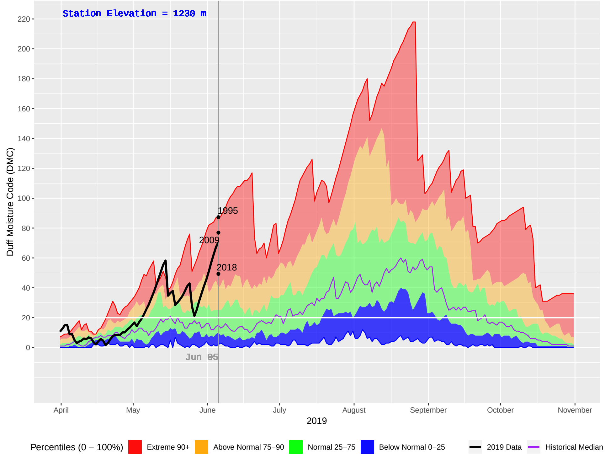
SLOCAN (406) : Historical (1992–2018), Current (2019) Daily Duff Moisture Code (DMC)
