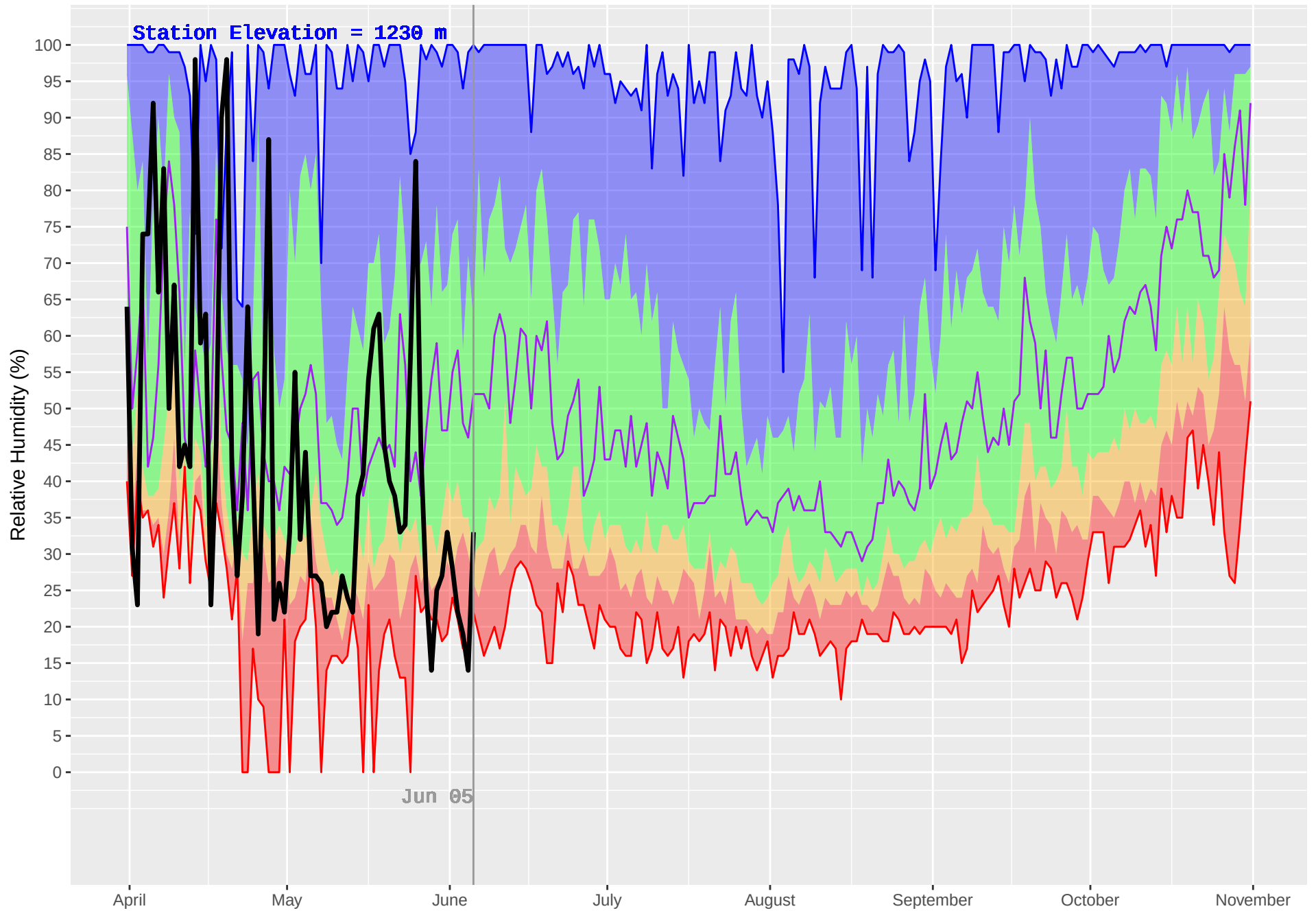
SLOCAN (406) : Historical (1992–2018) and Current (2019) Daily Relative Humidity
