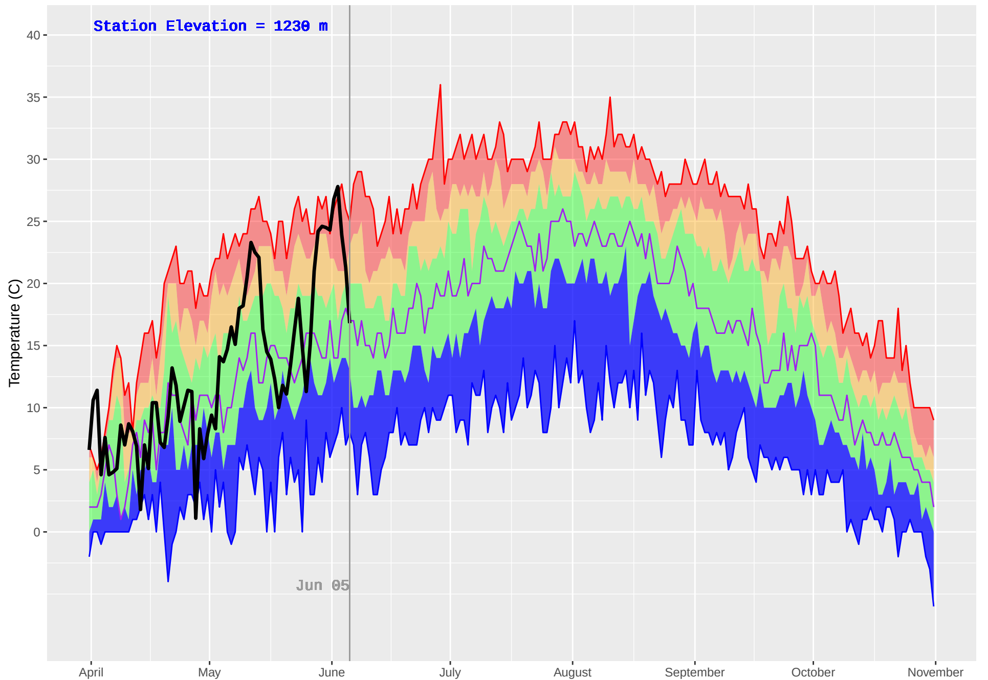
SLOCAN (406) : Historical (1992–2018) and Current (2019) Daily Temperature
