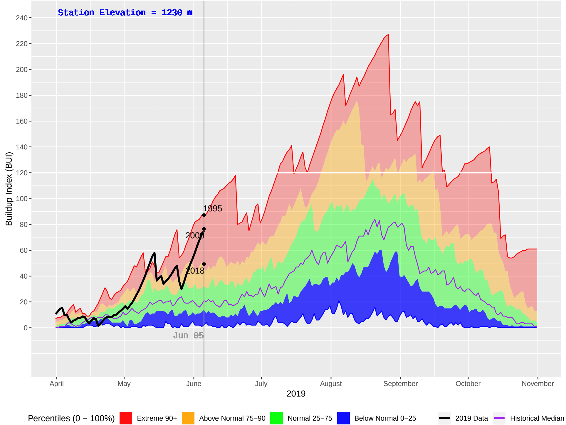
SLOCAN (406) : Historical (1992–2018), Current (2019) Daily Buildup Index (BUI)
