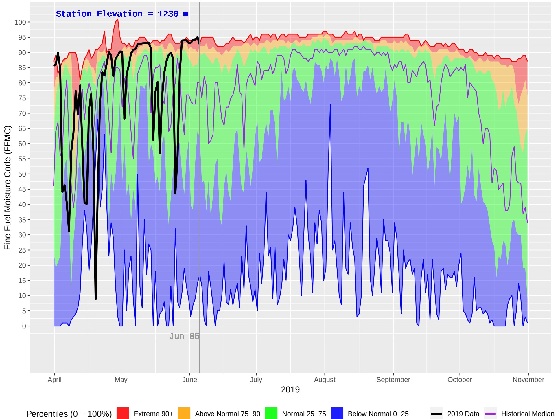
SLOCAN (406) : Historical (1992–2018) and Current (2019) Daily Fine Fuel Moisture Code (FFMC)
