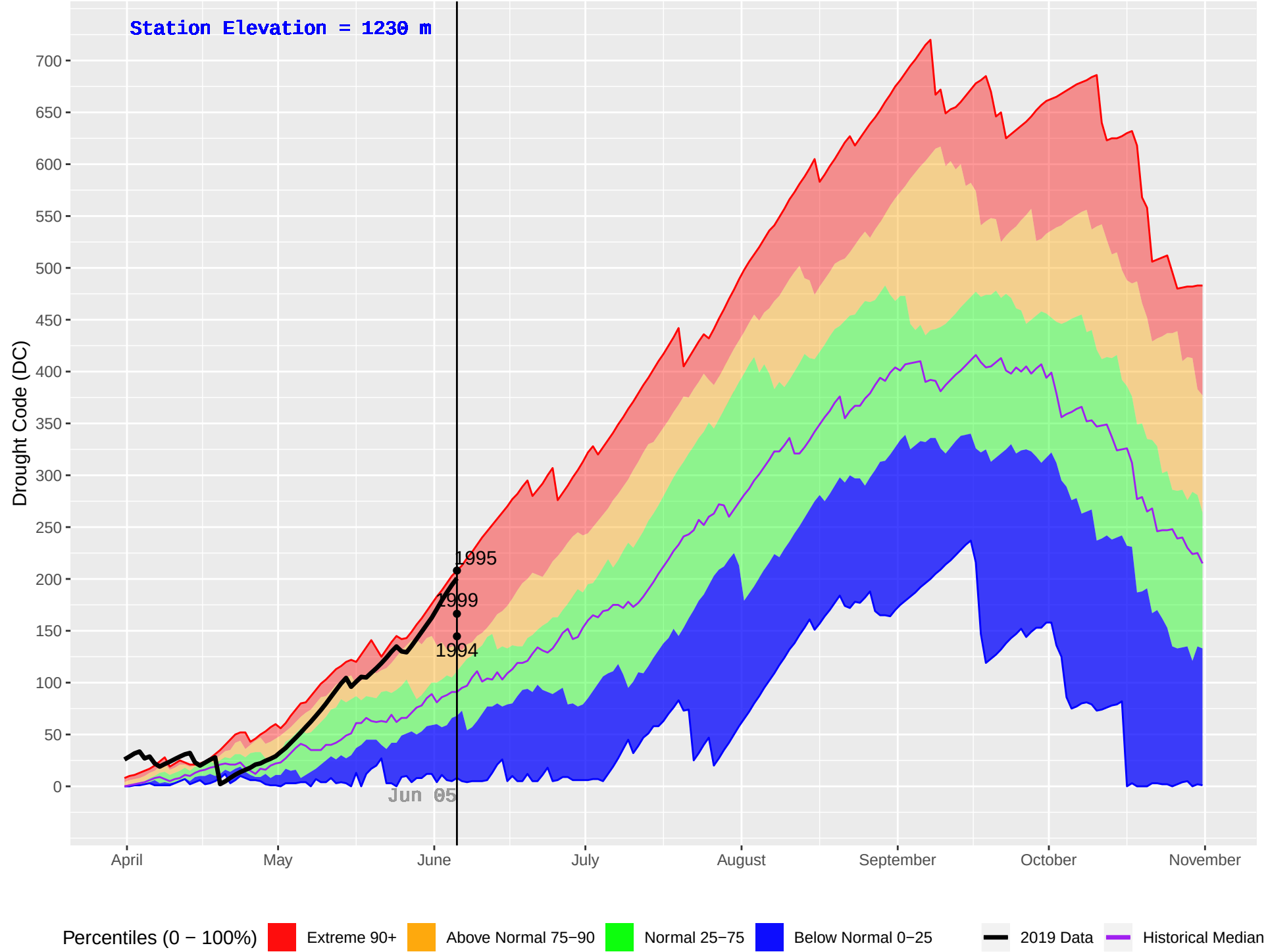
SLOCAN (406) : Historical (1992–2018) and Current (2019) Daily Drought Code (DC)
