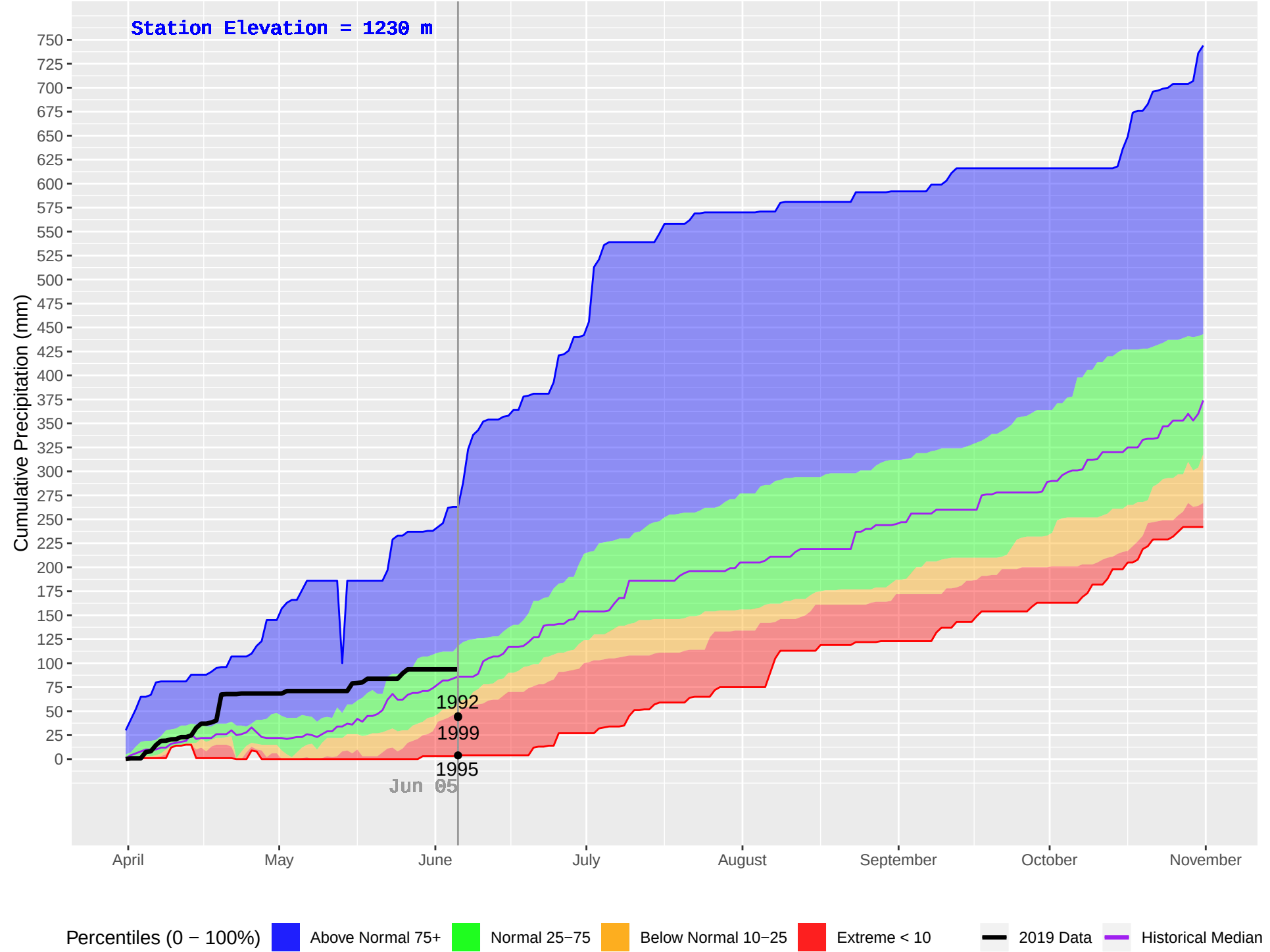
SLOCAN (406) : Historical (1992–2018), Current (2019) Daily Cumulative Precipitation
